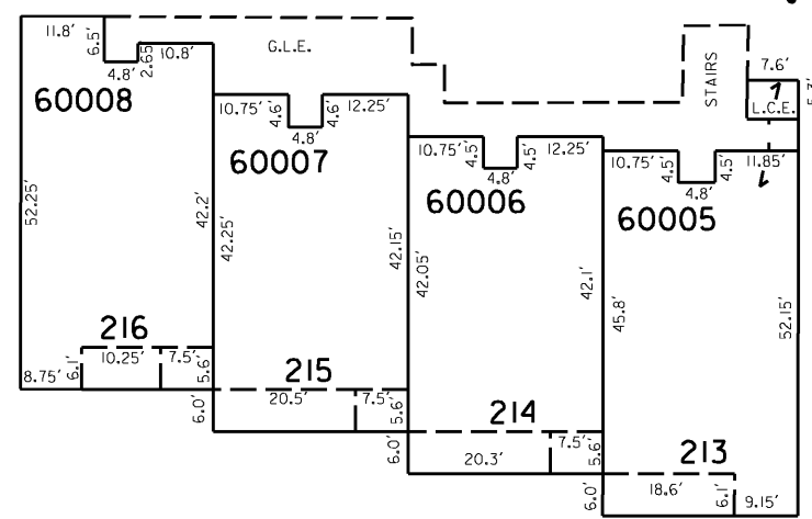
SECOND FLOOR
