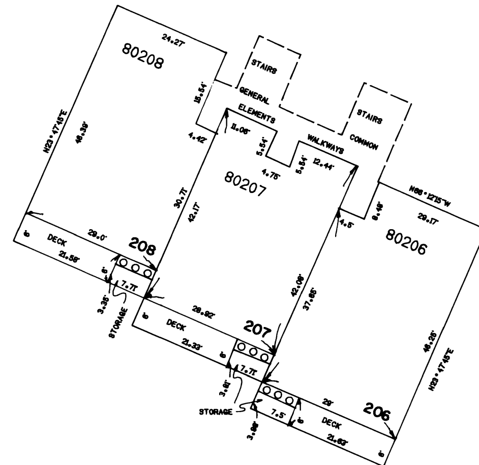
SECOND FLOOR PACIFIC VISTA CONDOMINIUM 1" - 20'
